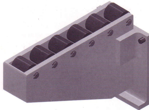
BOLSTER EXTENSIONS Bolt-on rail system to aid in die removal from the press
