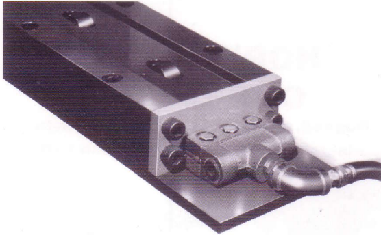
DI-GLIDE™ Quick Die Change System The heavy-duty pneumatic die lifting system for dies up to 160,000 lbs.
